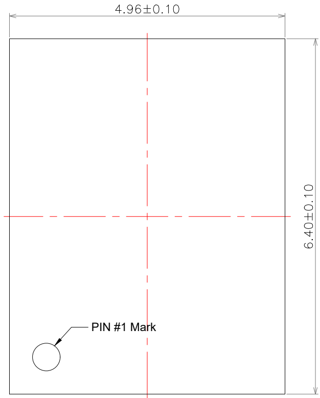
TOP VIEW
